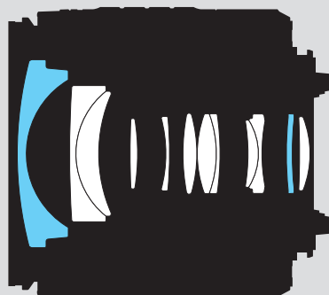
■: Aspherical lens elements
