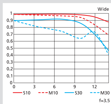
MTF Charts
